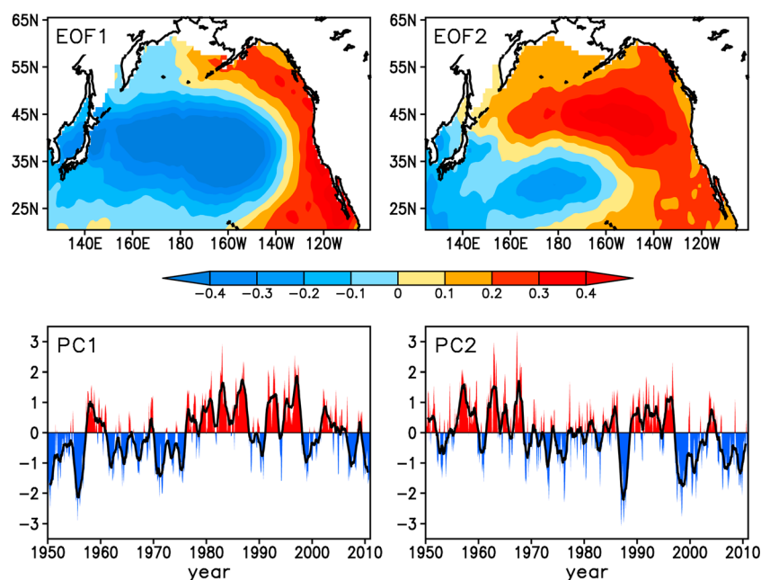
Figure 1. Spatial patterns and corresponding PCs of the first two leading EOF modes of the North Pacific (124.5°E–100.5°W, 20.5°N–65.5°N) monthly SSTA field (after removing the monthly mean global average SSTA). Monthly values of PC1 and PC2 time series are indicated by colored bars (red, positive and blue, negative) with a 13 month running mean overlain (bold lines).
