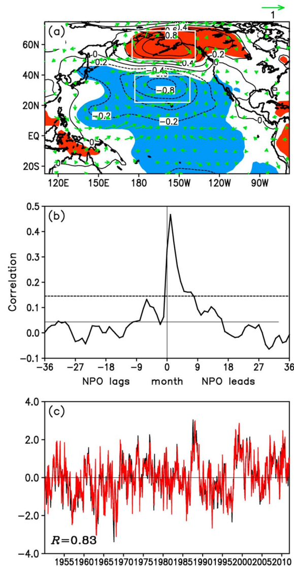
Figure 3. (a) Pacific SLP (mbar; contours) and surface wind ( \text{m s}^{-1} ; vectors) anomalies regressed on the VMI. The two white boxes denote the locations of the northern ( 175^{\circ}\text{E} – 138^{\circ}\text{W} , 50^{\circ}\text{N} – 69^{\circ}\text{N} ) and southern ( 177^{\circ}\text{E} – 142^{\circ}\text{W} , 22^{\circ}\text{N} – 40^{\circ}\text{N} ) poles of the NPO, respectively; the difference between the normalized SLP anomalies averaged over each pole is used to define the NPOI. Positive (red) and negative (blue) SLP anomalies, with regression coefficients significant at the 95% level, are shaded; only surface wind vectors significant at the 95% level are shown. (b) Lead-lag correlation coefficients between the raw monthly VM and NPO indices; the horizontal dashed line indicates the 99.9% significance level. (c) Observed VMI (black line) and reconstructed VMI (red line) using an AR1 model forced by the NPOI. The correlation coefficient ( R ) between the monthly values of observed and reconstructed VM indices is 0.83, significant at the 99.9% level.
