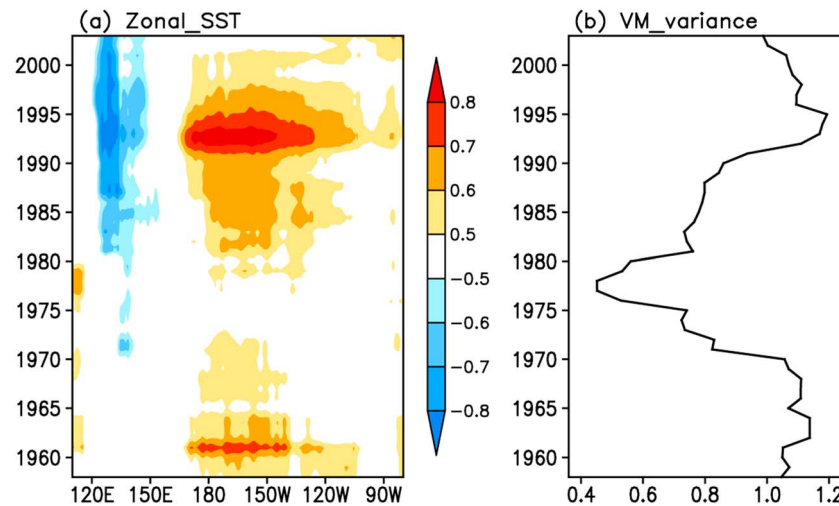
Figure 12. (a) The 15 year moving correlations between the FMA(0) VMI and JFM(+1) SSTs averaged over 5°S–5°N for the period 1950–2011. Areas with correlation significant at the 95% level are shaded. (b) Time series of running SD of the FMA(0) VMI calculated within a 15 year window that moves year by year for the period 1950–2011.
